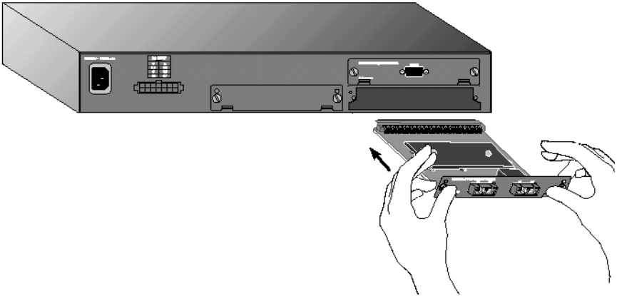
Figure 5 Installing the Expansion Module
