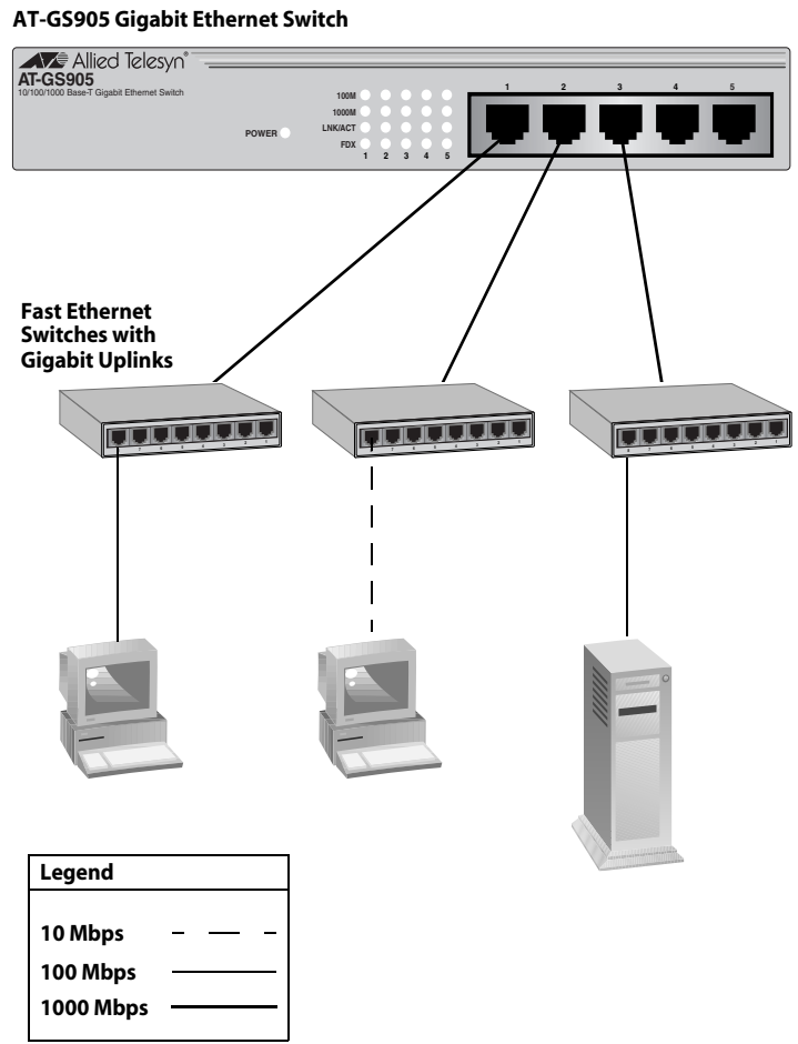
Figure 4 Collapsed Backbone - Hub Topology
