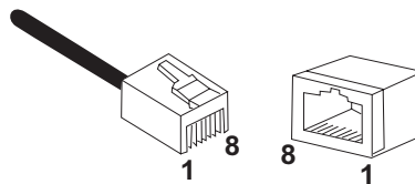
Figure 10 RJ-45 Connector and Port Pin Layout
