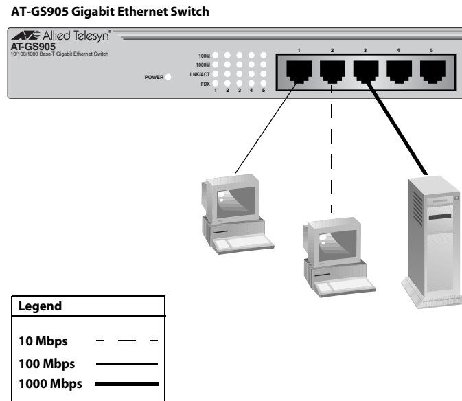
Figure 3 Power Workgroup Topology
