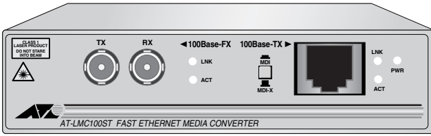
Figure 2 AT-LMC100ST Converter - Front Panel
