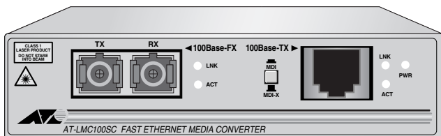
Figure 1 AT-LMC100SC Model Converter - Front Panel
