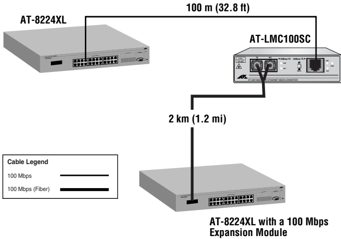
Figure 4 Standalone Topology
