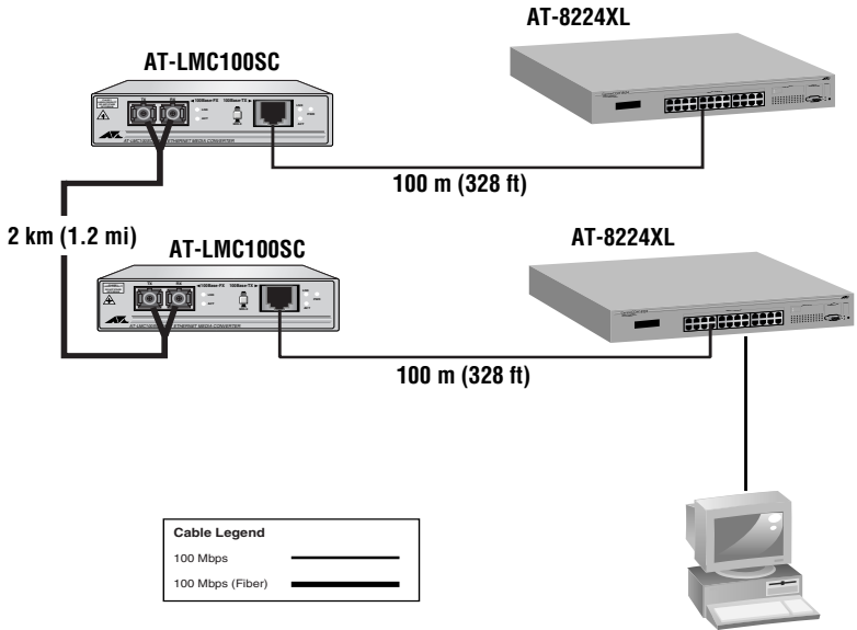
Figure 5 Back-to-Back Topology
