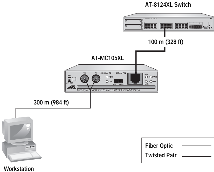
Figure 4 Standalone Topology
