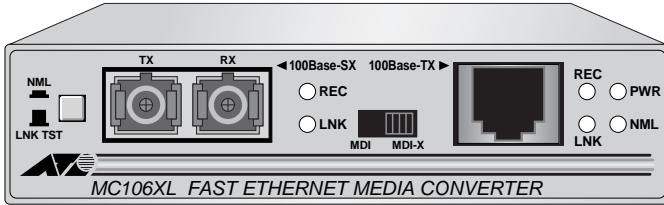
Figure 2 AT-MC106XL Front Panel (SC Connector)
