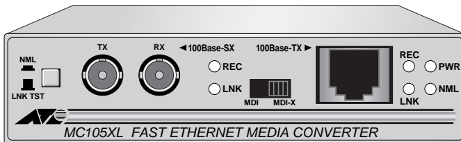
Figure 1 AT-MC105XL Front Panel (ST Connector)
