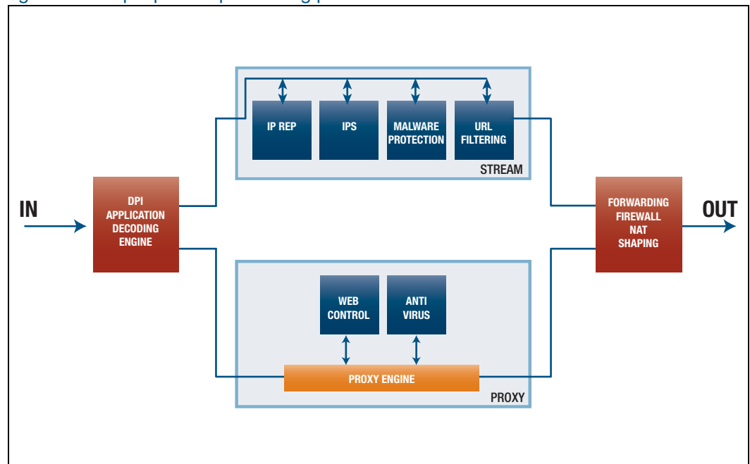
Figure 5: Multiple parallel processing paths
