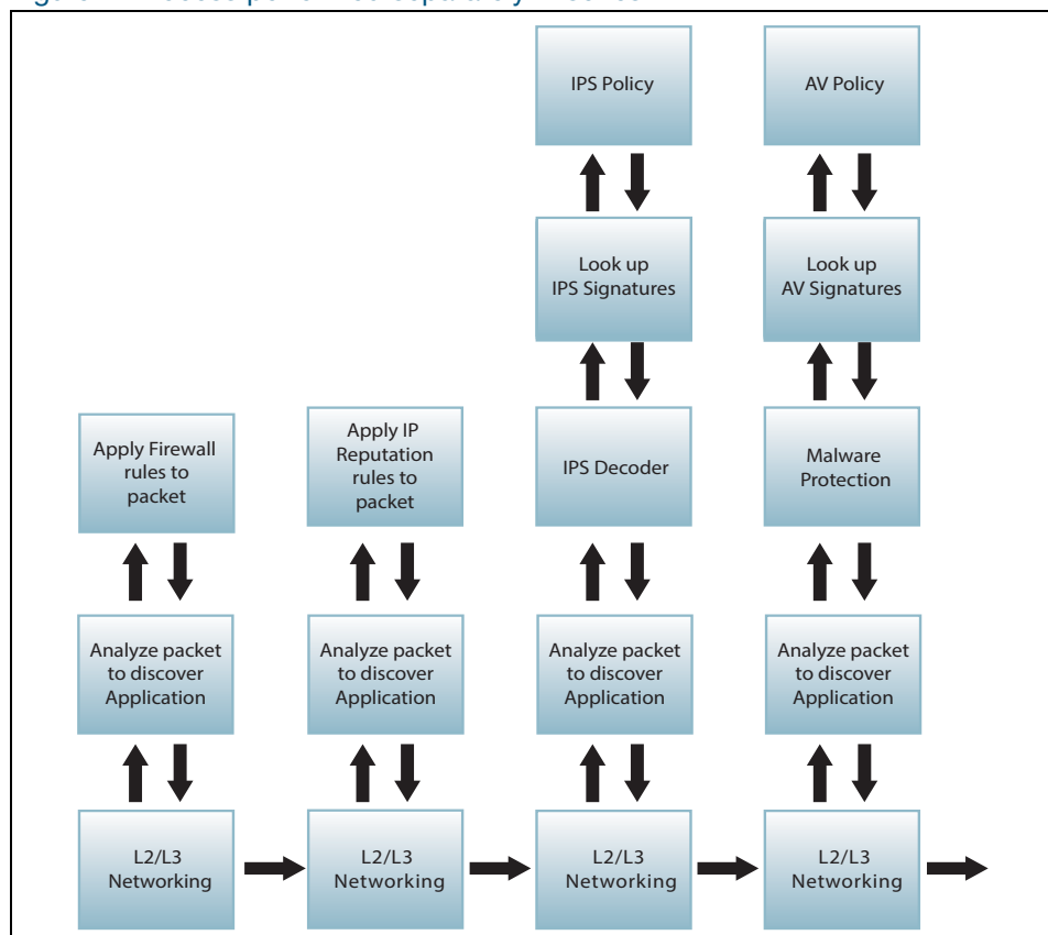
Figure 4: Process performed separately in series
