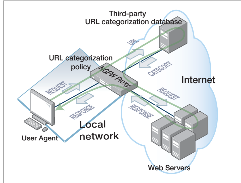
Figure 3: Web control
