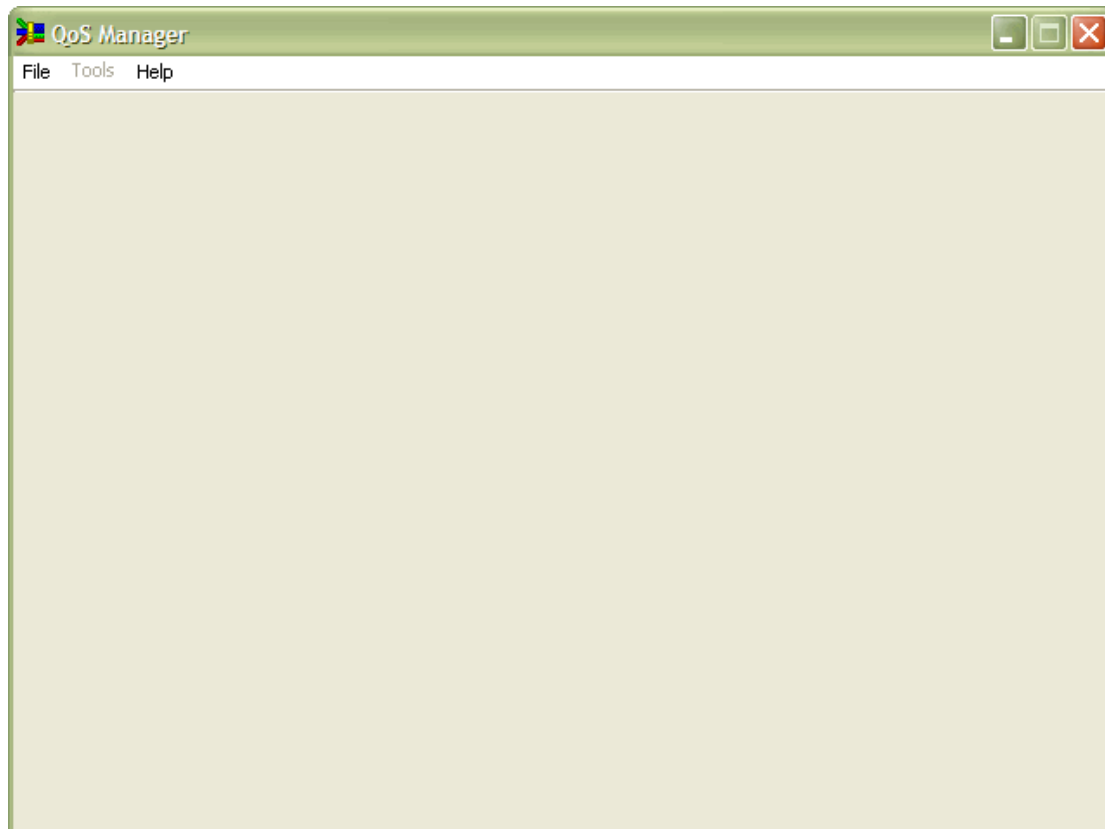
Initial Window
