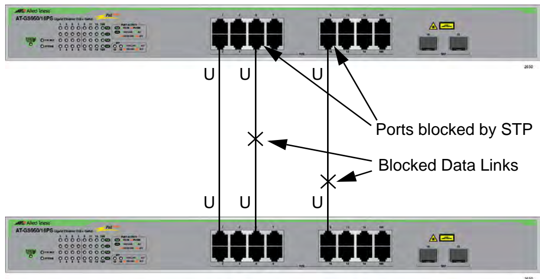
Figure 26. STP and VLAN Fragmentation with Untagged Ports
