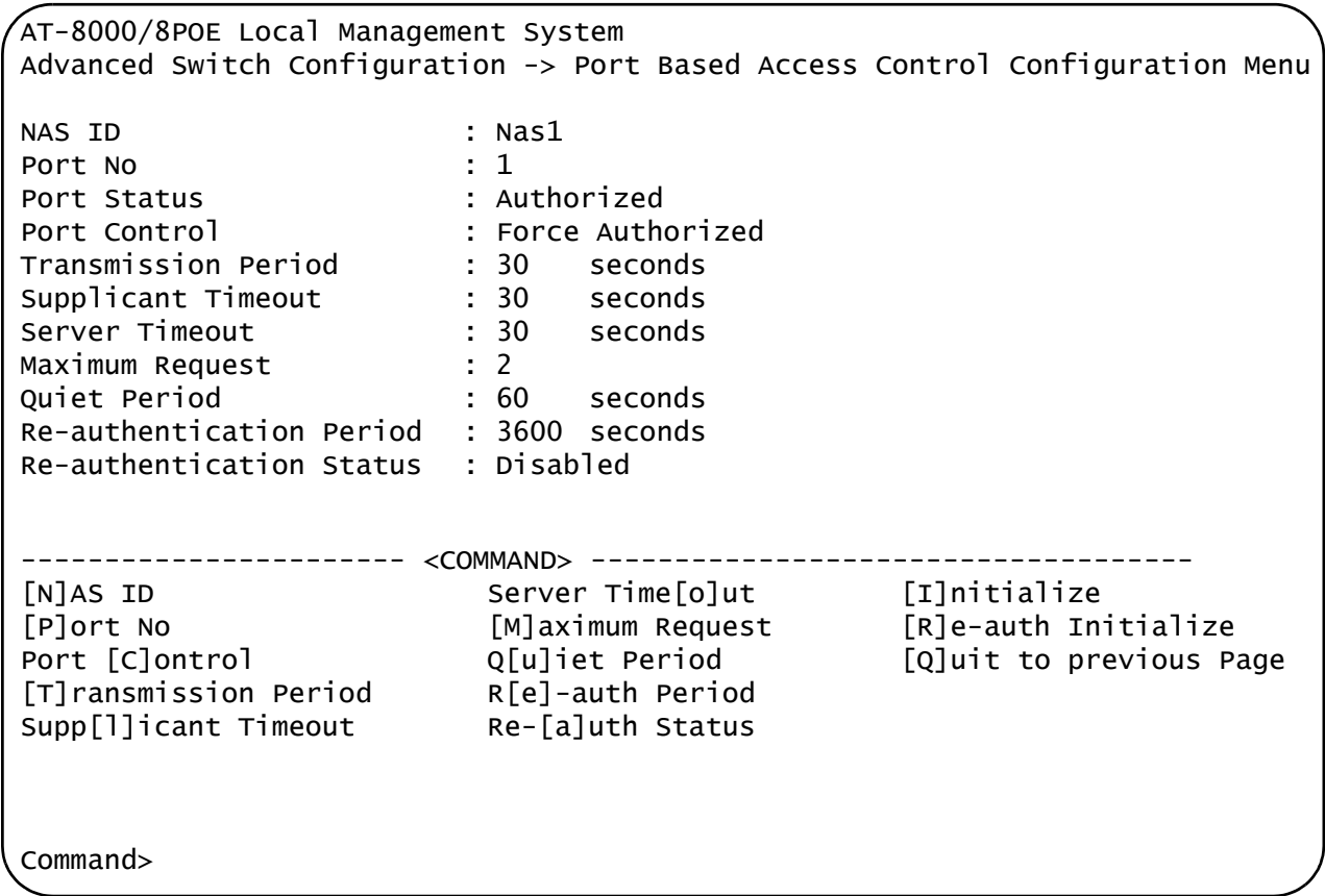
Figure 40. Port Based Access Control Configuration Menu
