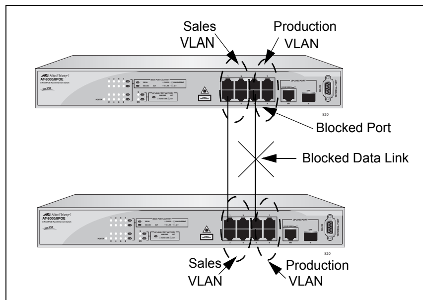
Figure 33. VLAN Fragmentation
