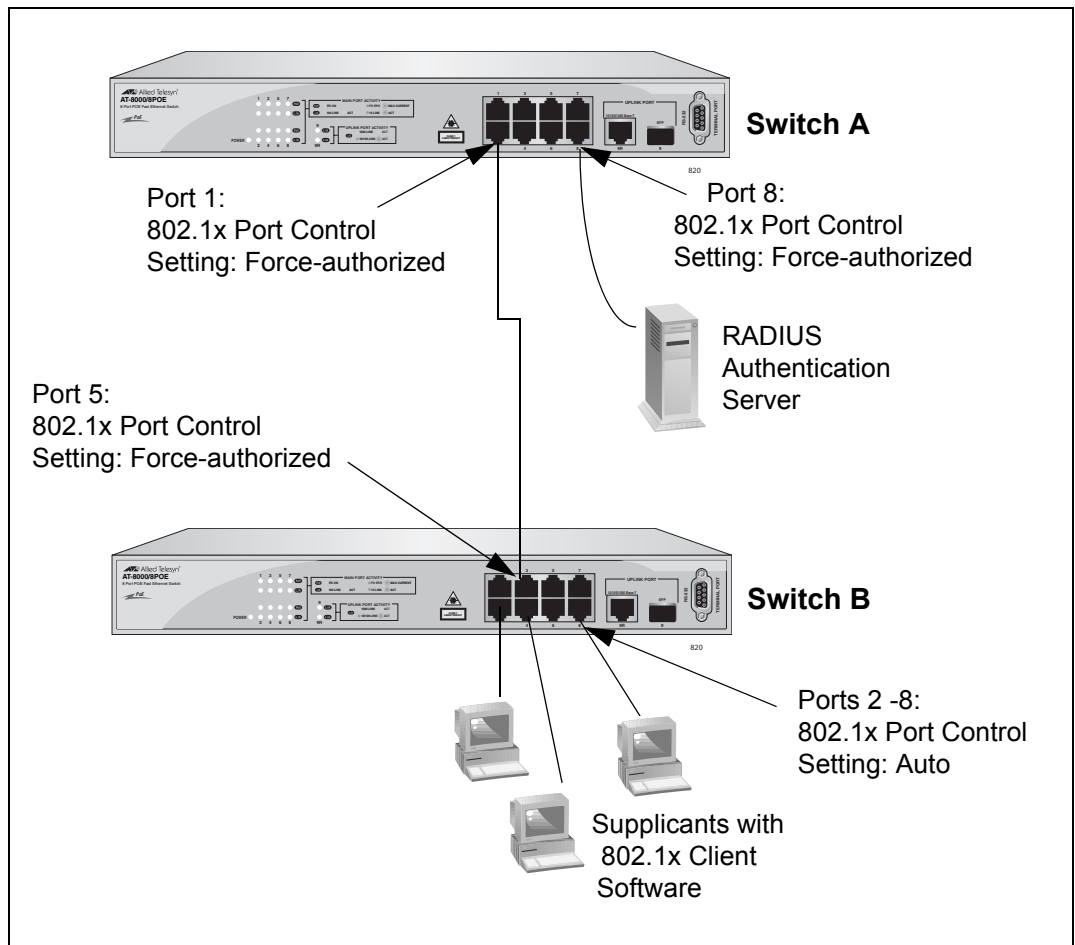
Figure 39. Authentication Across Multiple Switches
