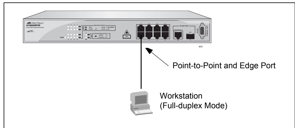
Figure 32. Point-to-Point and Edge Port
