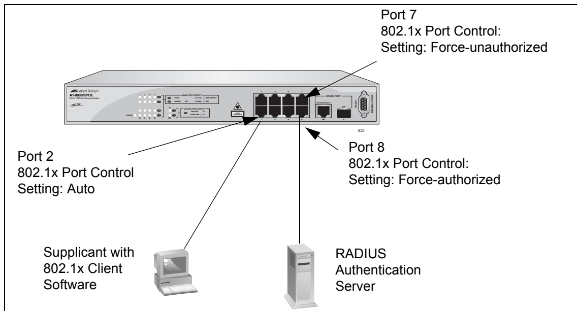
Figure 38. Example of the Authenticator Role
