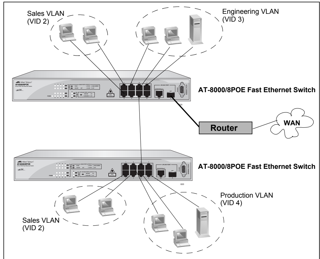
Figure 20. Example of a Tagged VLAN
