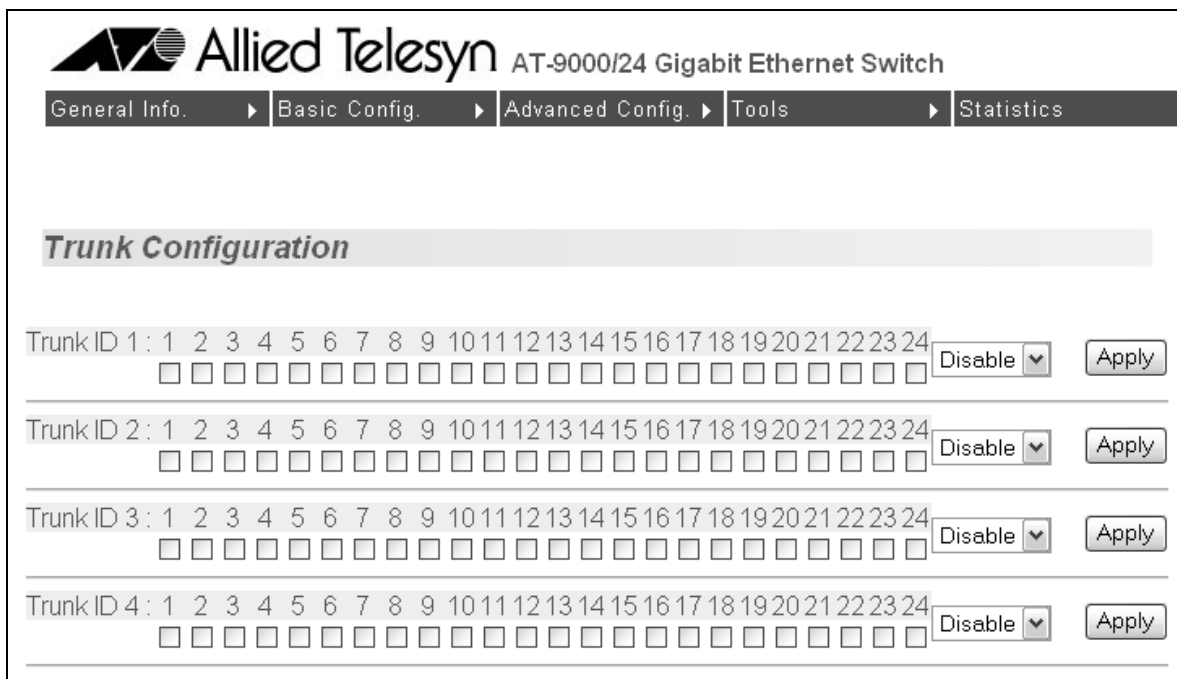
Figure 71. Trunk Configuration Page
