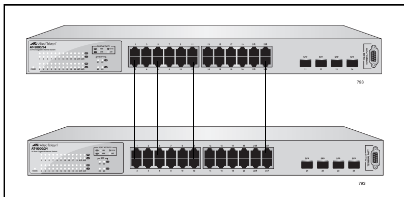
Figure 19. Static Port Trunk Example
