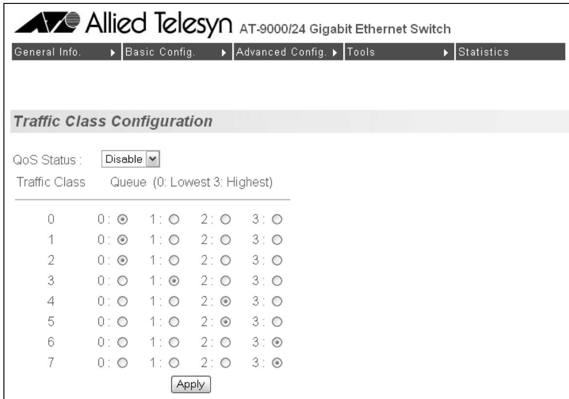
Figure 80. Traffic Class Configuration Page
