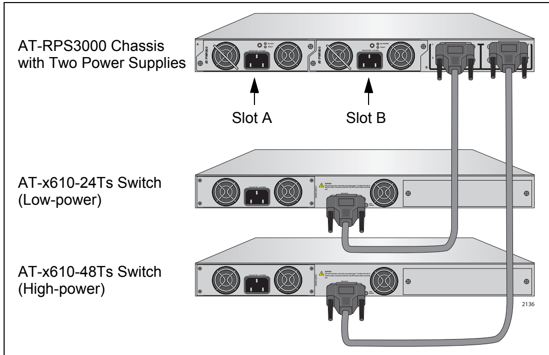
Figure 11. Example of Low-power and High-power Switches
