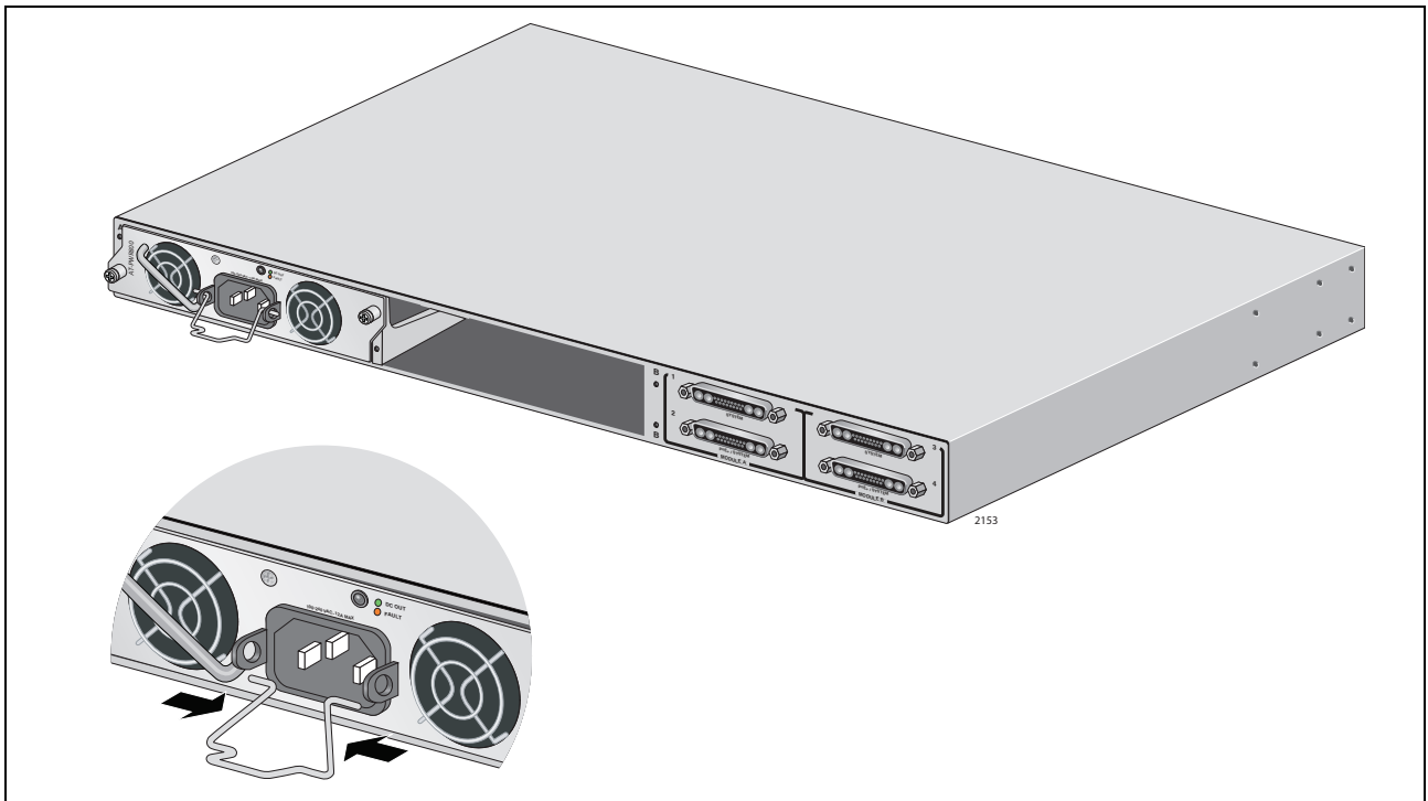
Figure 42. Installing a Power Cord Retaining Clip
