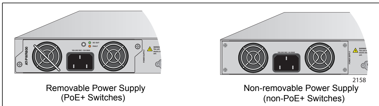
Figure 6. Removable and Non-removable Power Supply Modules in x610 Switches
