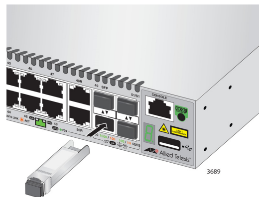
Figure 41. Installing an SFP Transceiver
