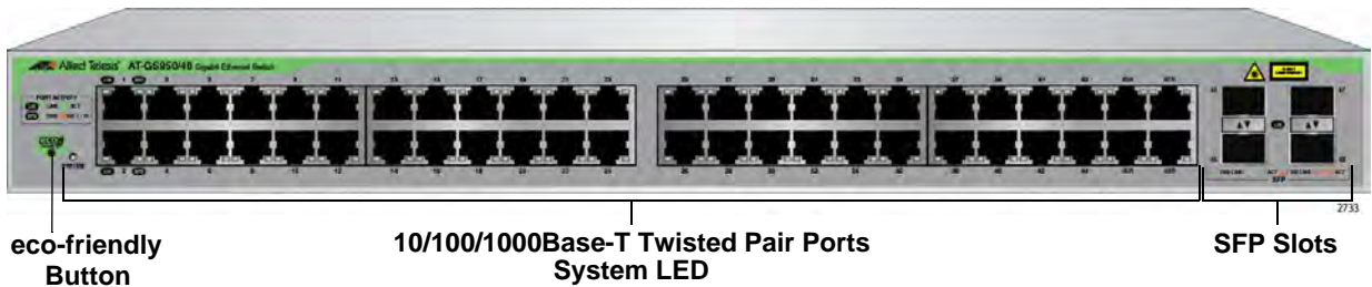
Figure 1. AT-GS950/8, AT-GS950/16, AT-GS950/24 and AT-GS950/48 Front Panels
