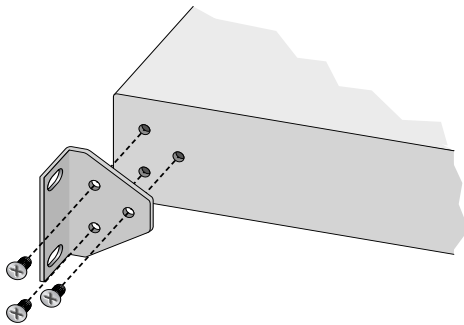
Figure 8 Installing the Mounting Bracket
