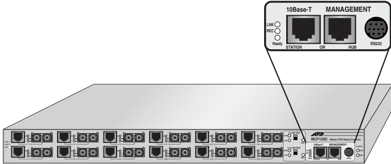
Figure 6 10Base-T, Management, and RS-232 Ports
