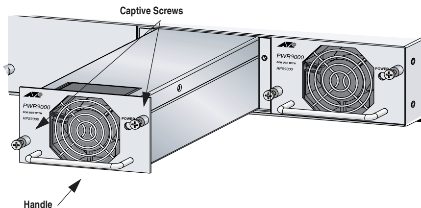
Figure 1: Captive mounting screws on the AT-PWR9000
