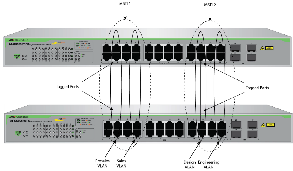
Figure 157. Multiple VLANs in an MSTI
