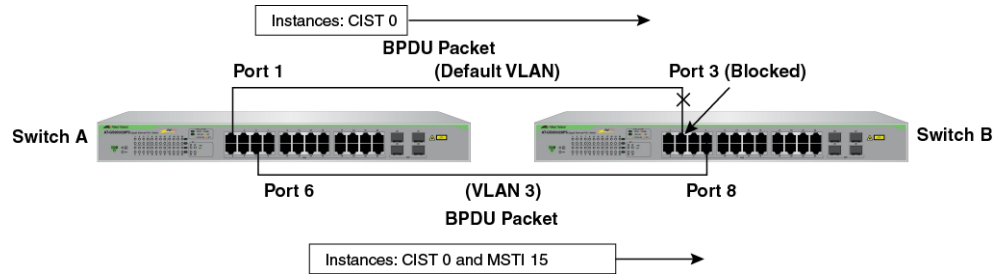
Figure 159. CIST and VLAN Guideline - Example 2
