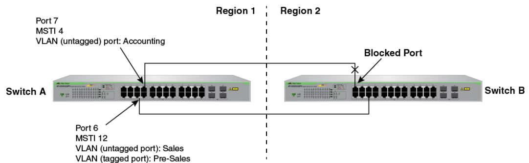
Figure 160. Spanning Regions - Example 1
