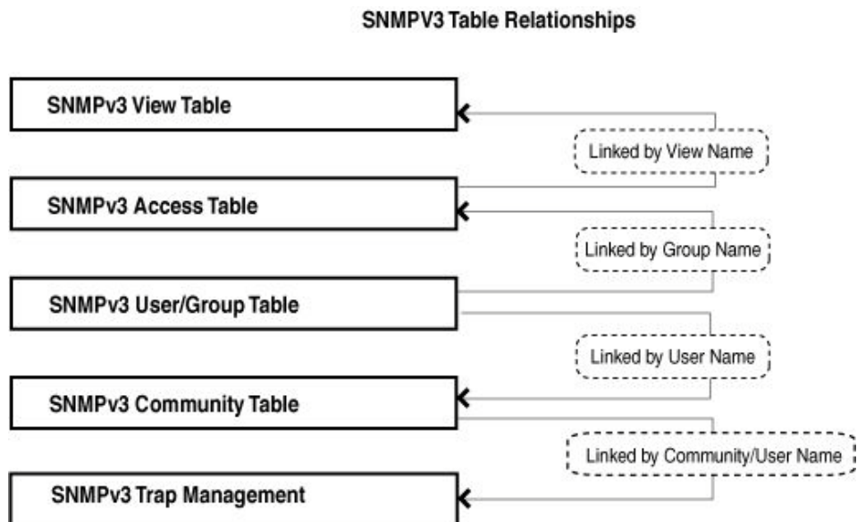
Figure 84. SNMPv3 Table Relationships
