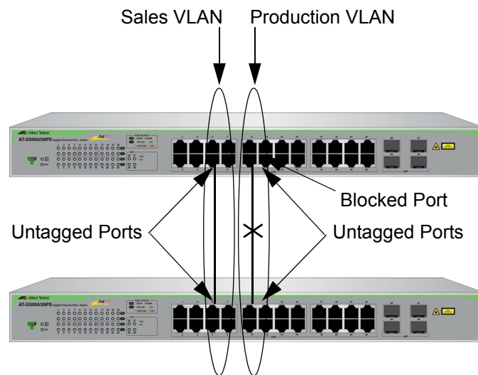
Figure 155. VLAN Fragmentation with STP or RSTP
