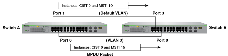
Figure 158. CIST and VLAN Guideline - Example 1
