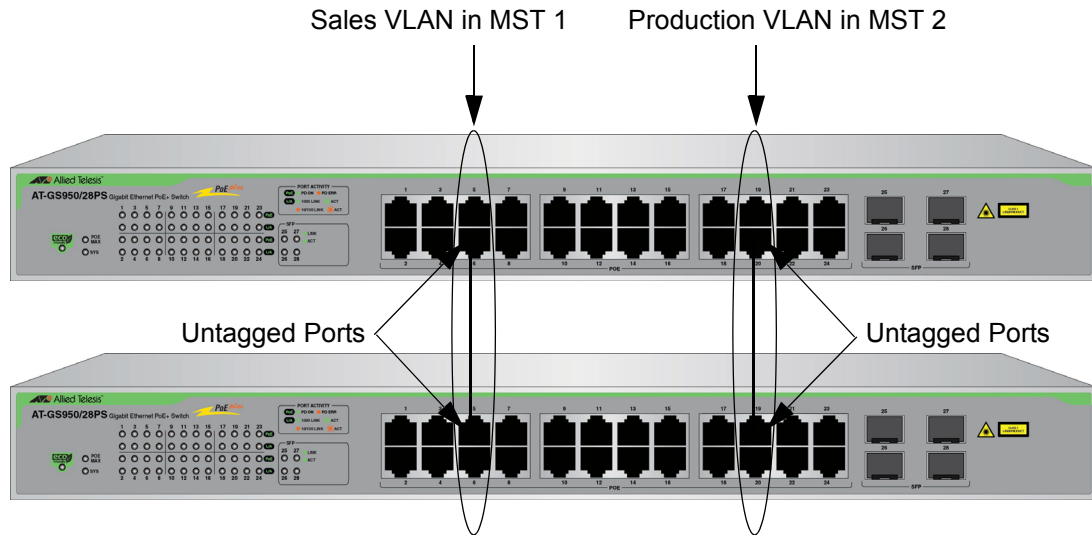
Figure 156. MSTP Example of Two Spanning Tree Instances
