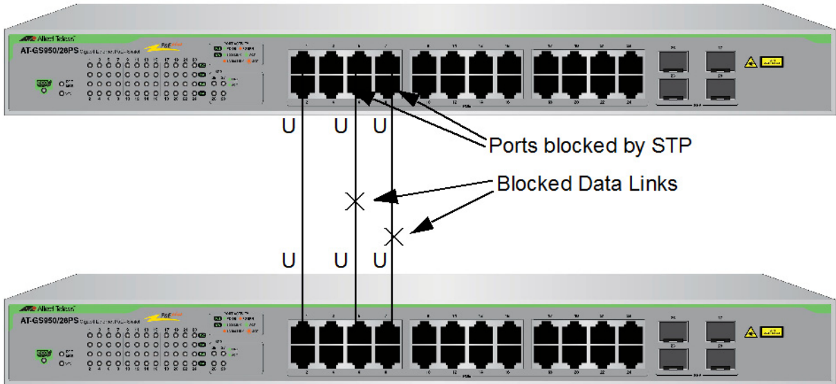
Figure 26. STP and VLAN Fragmentation with Untagged Ports
