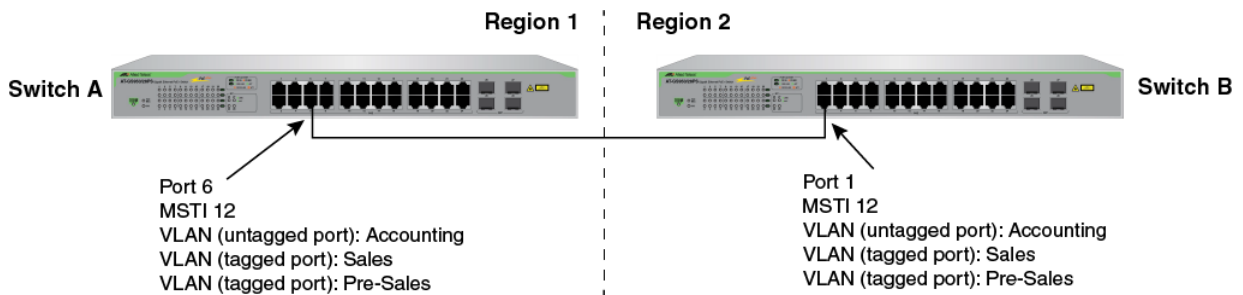
Figure 161. Spanning Regions without Blocking
