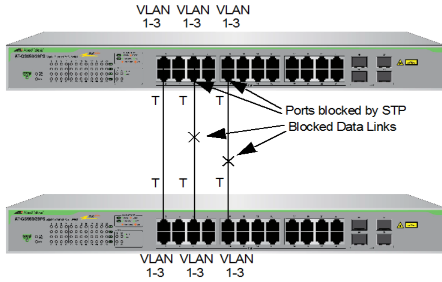
Figure 27. STP and VLAN Compatibility with Tagged Ports
