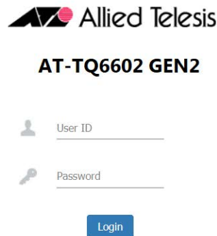
Figure 31. Login Prompt
