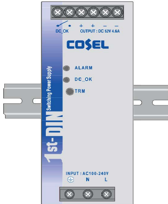
Figure 5. Vertical Installation
