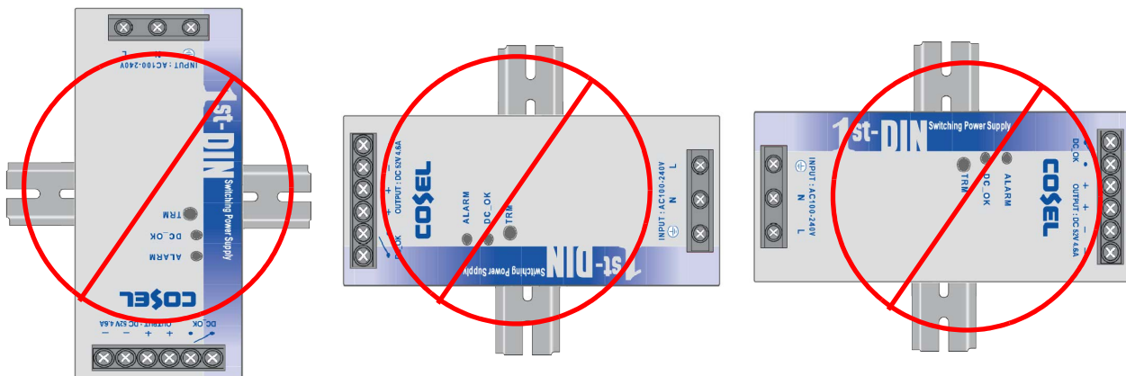
Figure 6. Unsupported DIN Rail Installations
