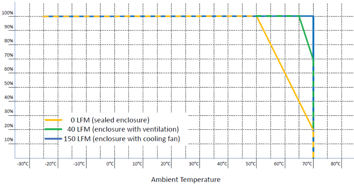
Figure 17. Derating Graph at 100Vac
