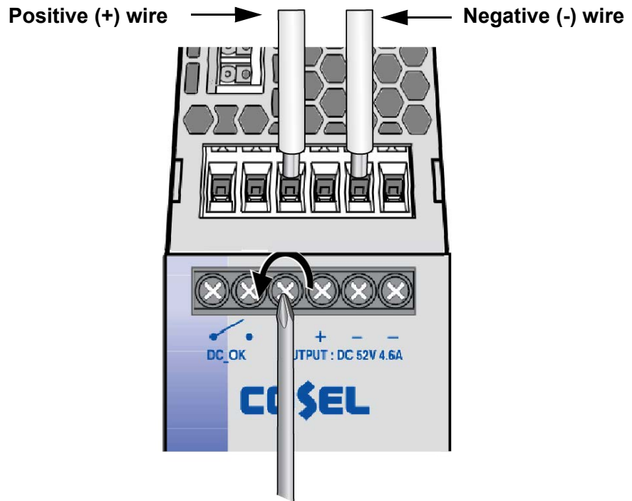
Figure 14. Installing DC Output Power Wires
