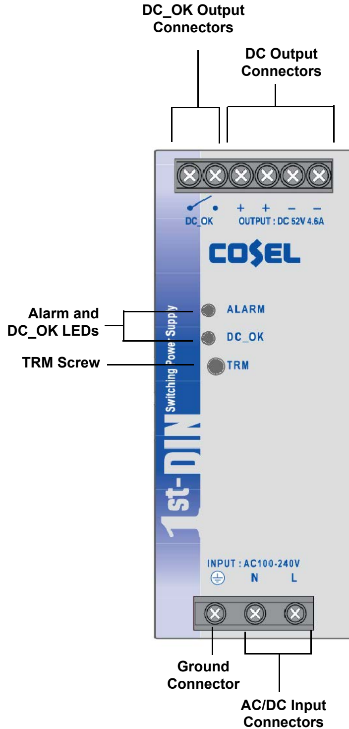
Figure 1. Front Panel
