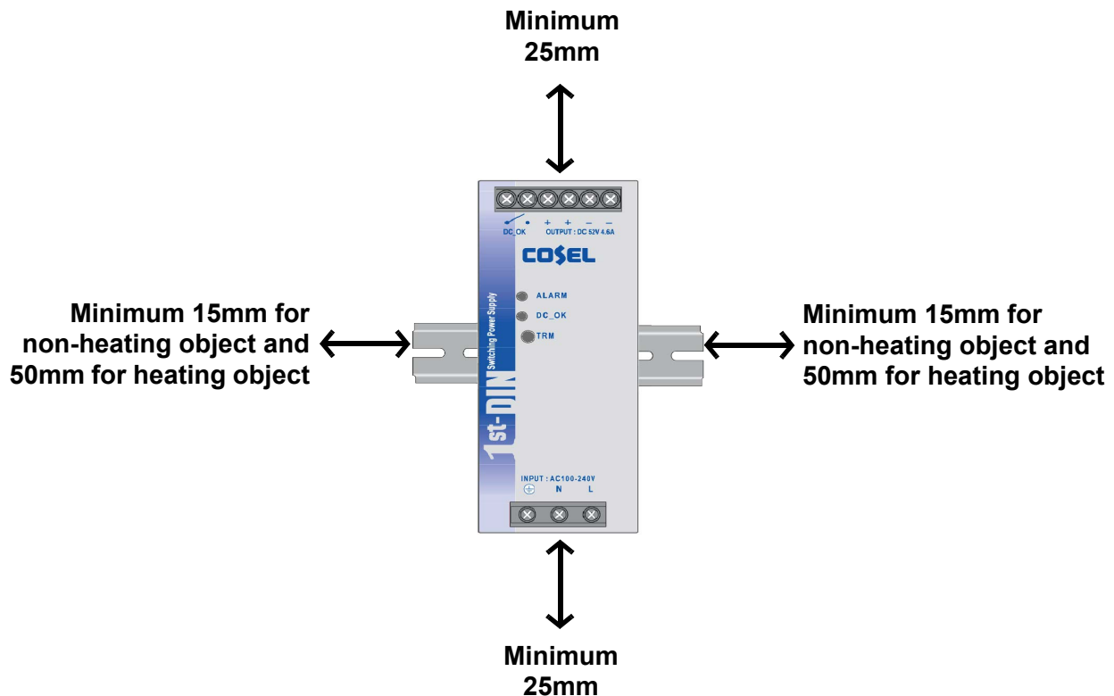
Figure 8. Minimum Spacing Requirements
