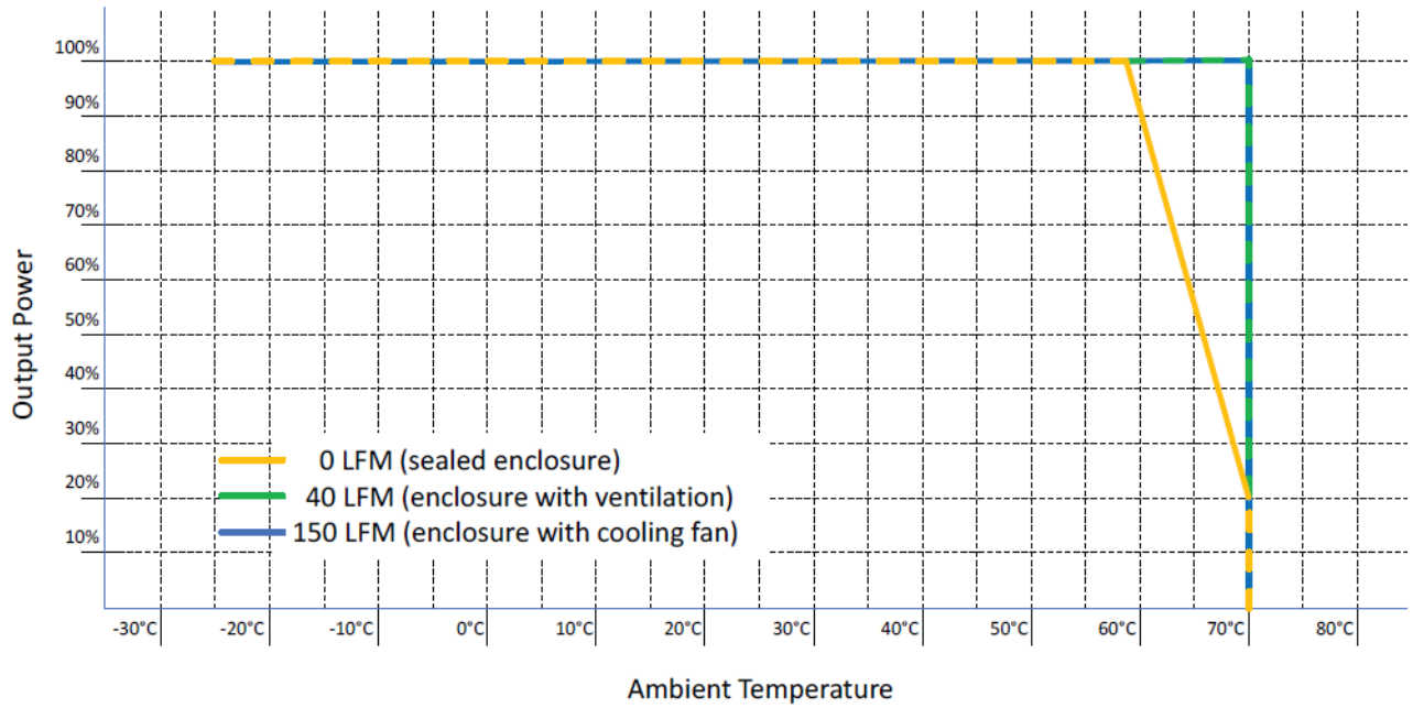
Figure 18. Derating Graph at 230Vac
