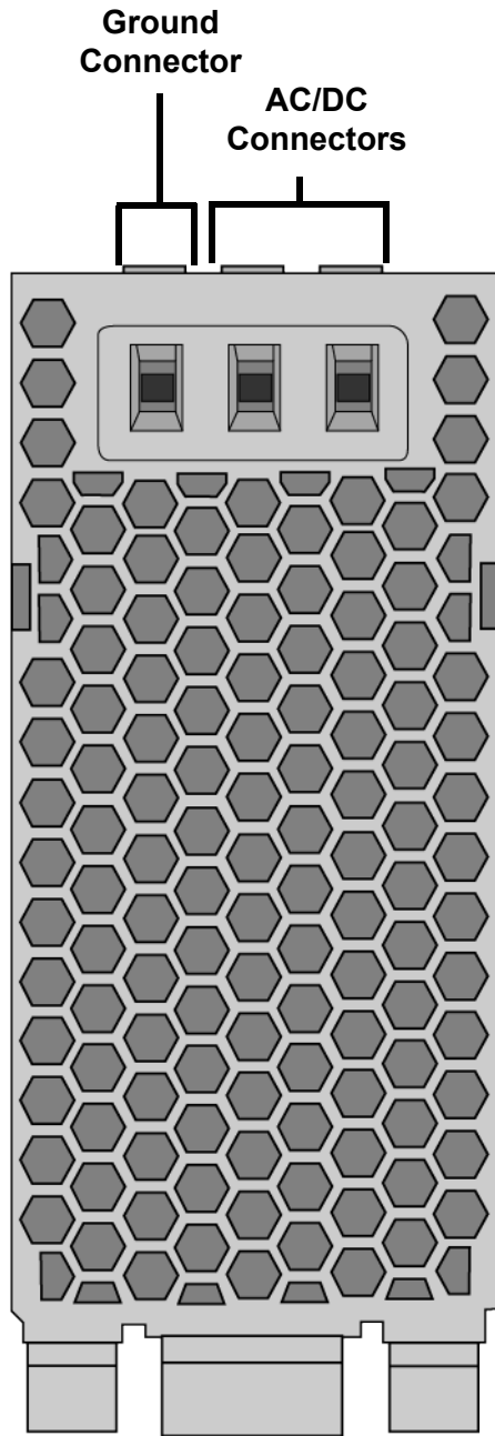
Figure 3. Bottom Panel
