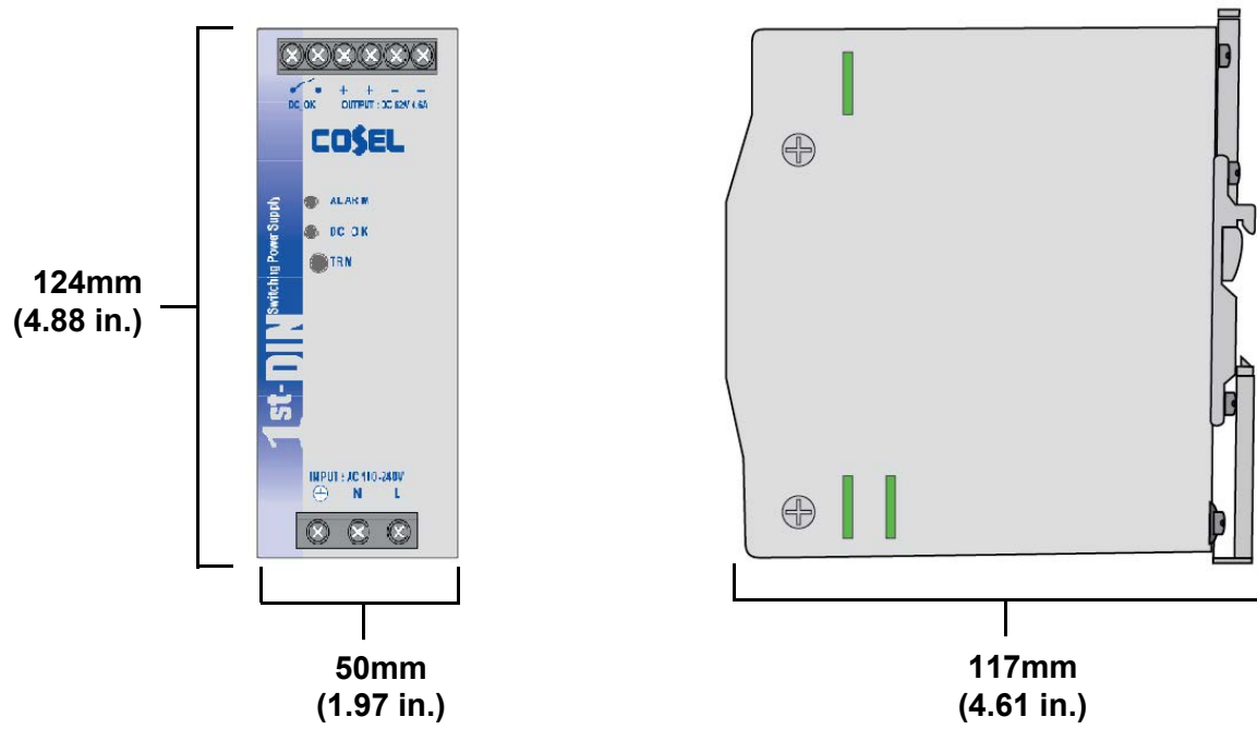
Figure 20. IE048-240 Power Supply Dimensions
