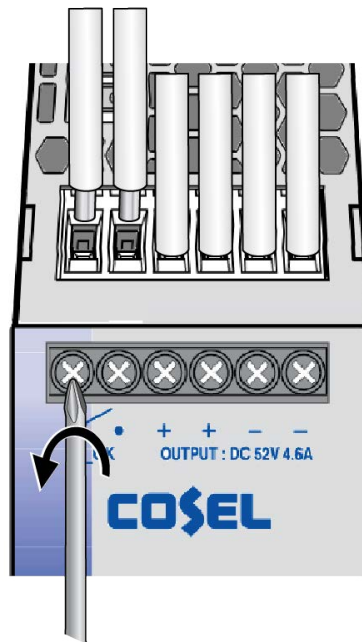
Figure 16. Wiring the DC_OK Connector
