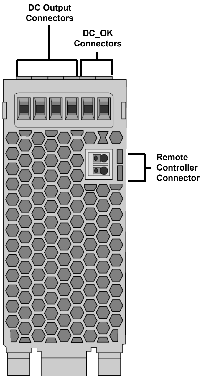
Figure 2. Top Panel
