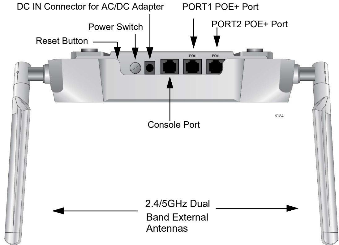
Figure 1. Components on the Back of the Access Point
