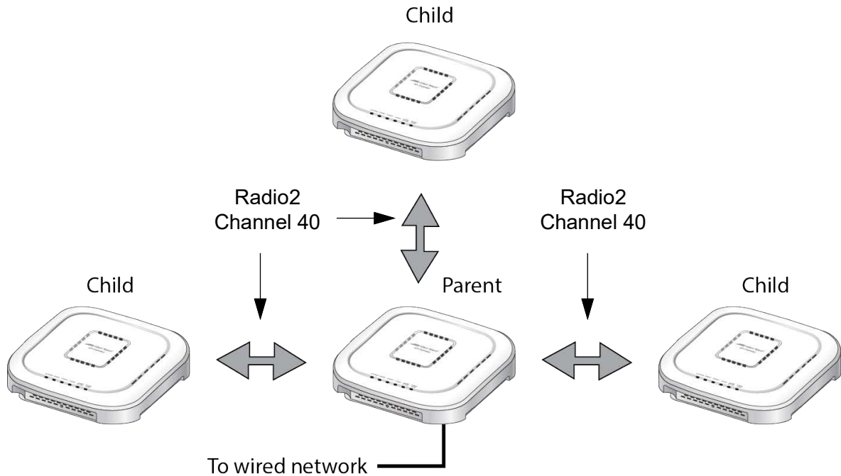
Figure 73. Example of Radio and Channel Assignments in a WDS Bridge
