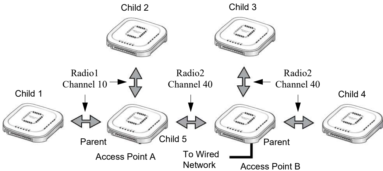
Figure 74. Example of an Access Point as Both Parent and Child
